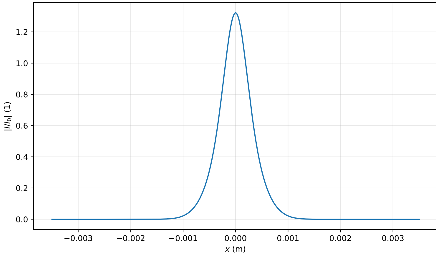
Intensity profile I(x, y = 0, z = 0.716m)/I_0 , P_{in}=1.0P_{cr} , artificial time
